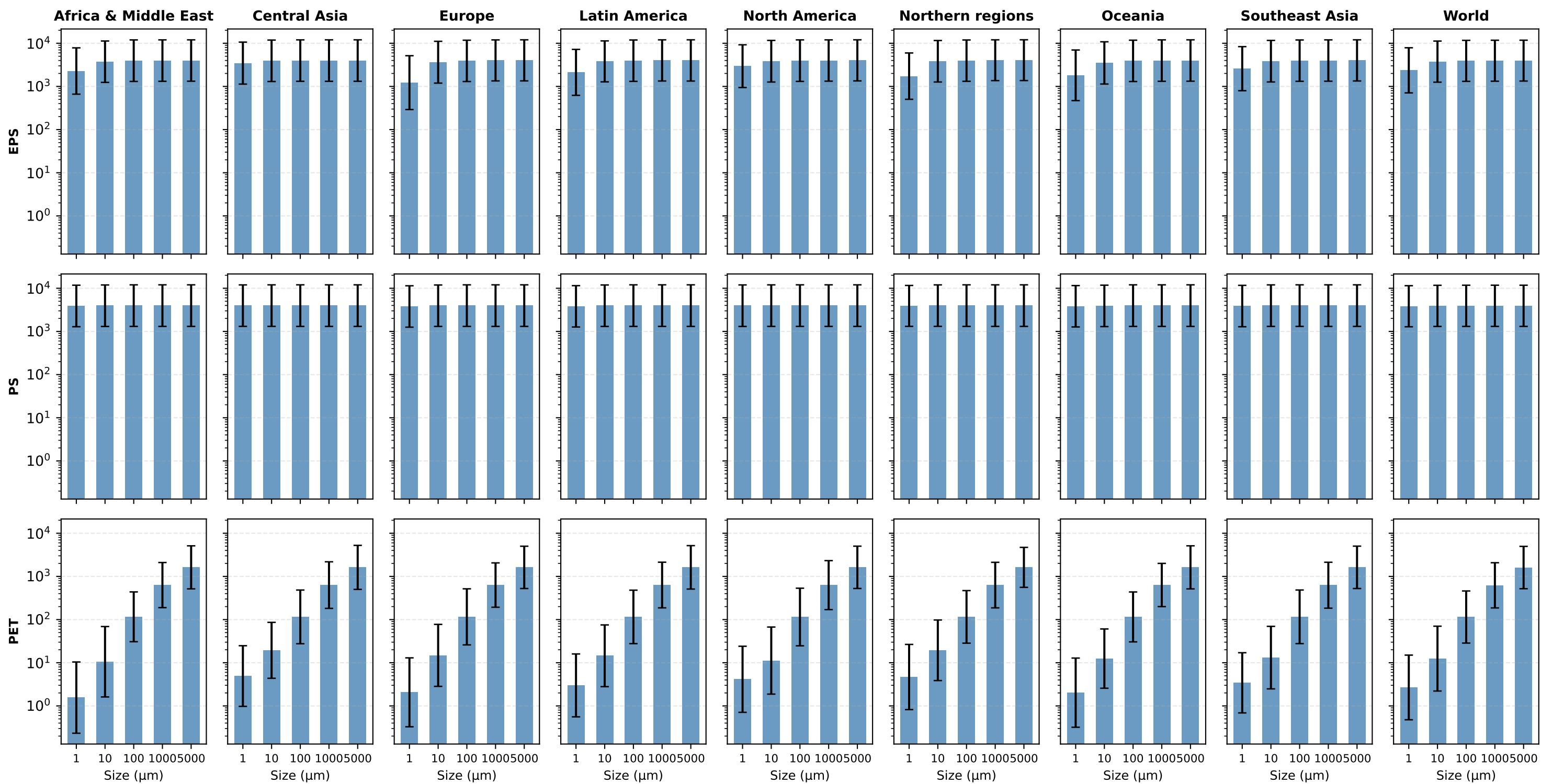
Endpoint characterization factor (PDF m2 yr/kg)
